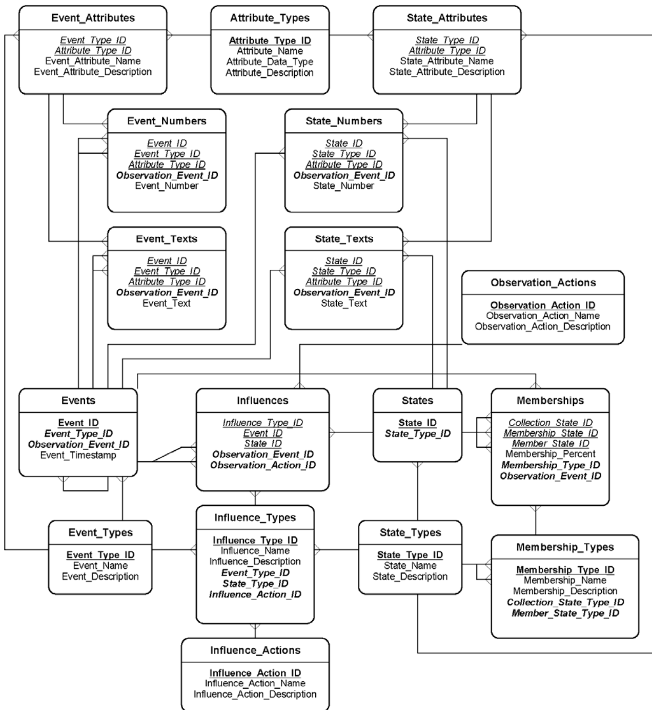
Figure 3: Entity-Relationship Diagram of SPEHR
